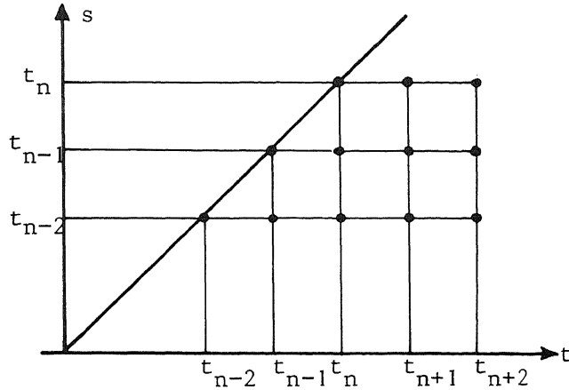
FIG. 1. Points in the (t, s) -plane needed in (2.5) for k = 2
