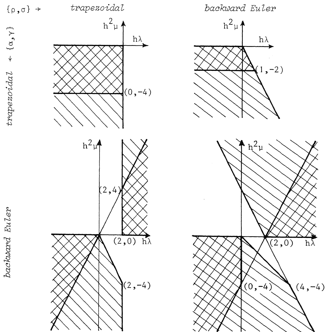
FIG. 2. Stability regions for MML(///) and ILM(\\) methods
